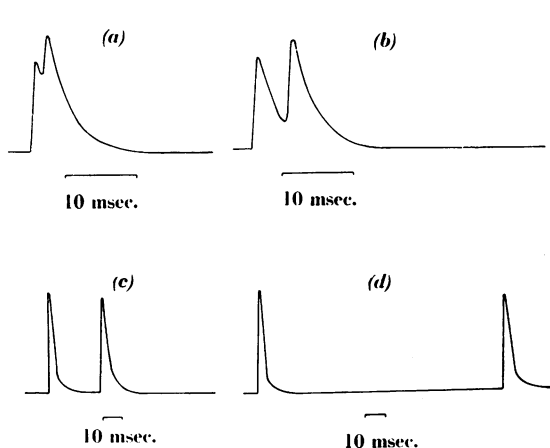
FIG. 5.—Cat, chloralose, gracilis. Records of endplate potentials after 75 \mu g. toxiferine I per kg. intravenously. Effect of paired shocks with different stimulus intervals: (a) 1.3 msec.; (b) 4.73 msec.; (c) 23.2 msec.; (d) 110 msec.
